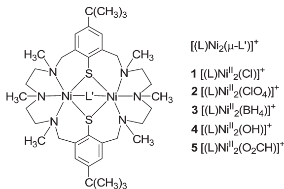
Scheme 1 Complexes 1–5.
